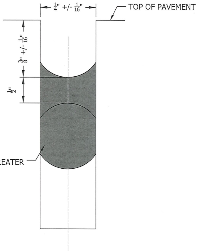
SILICONE JOINT SEALANT DETAIL
