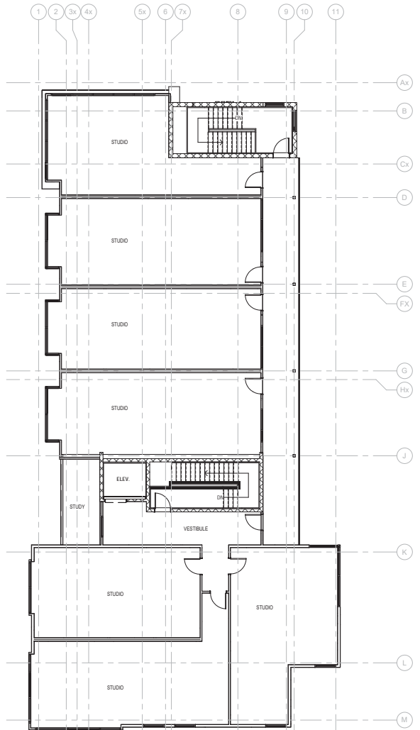
LEVEL 4 - NEW FLOOR PLAN 1/8" = 1'-0" NORTH
