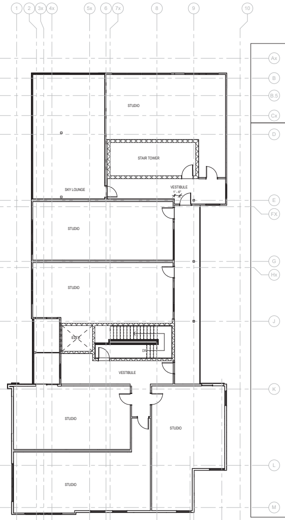
LEVEL 4 - NEW FLOOR PLAN 1/8" = 1'-0" NORTH
