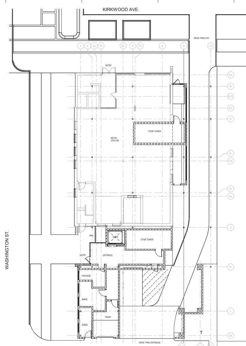
1 LEVEL 1 - NEW FLOOR PLAN 1/8" = 1'-0" NORTH
