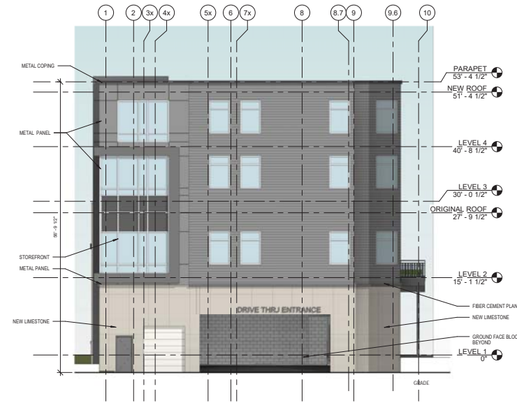
2 SOUTH ELEVATION A201 1/8" = 1'-0"
