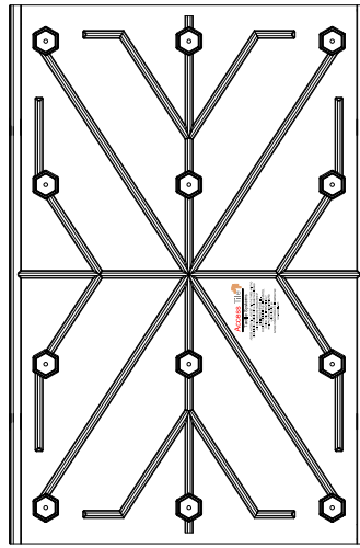
UNDERSIDE VIEW
