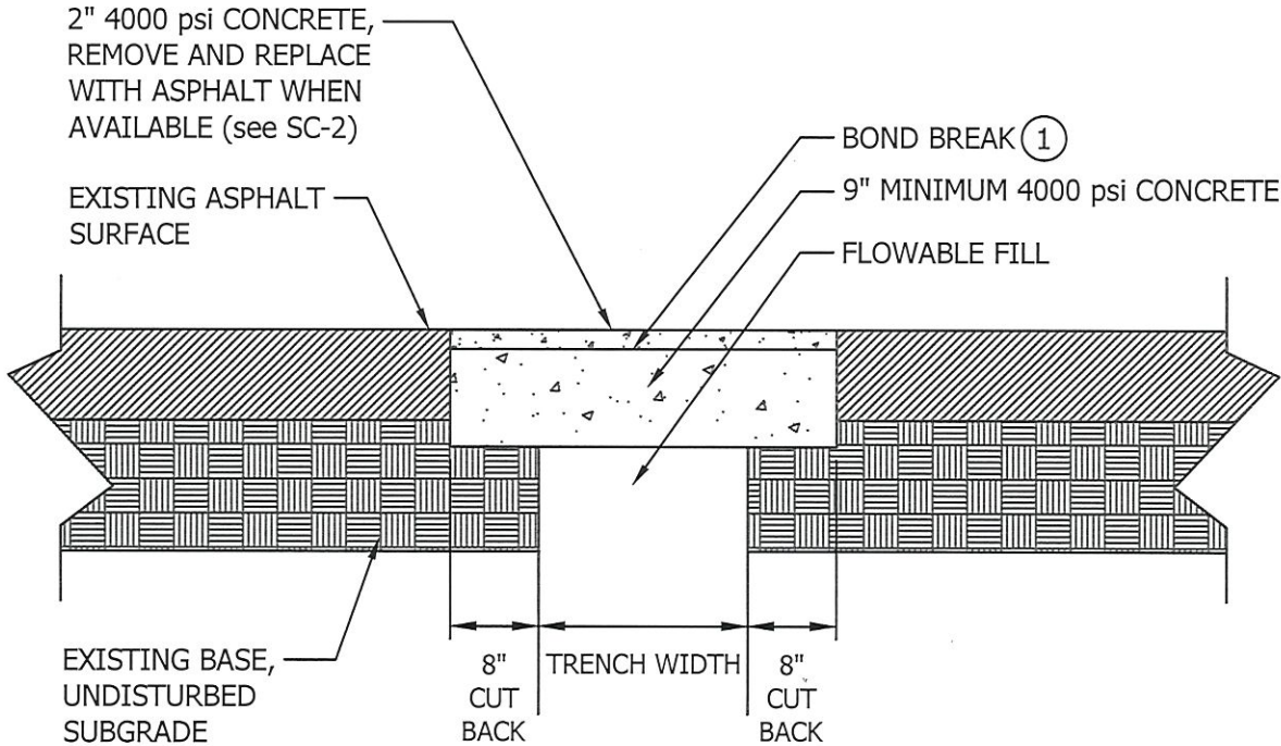
TEMPORARY STREET CUT REPAIR (Winter Repair)
