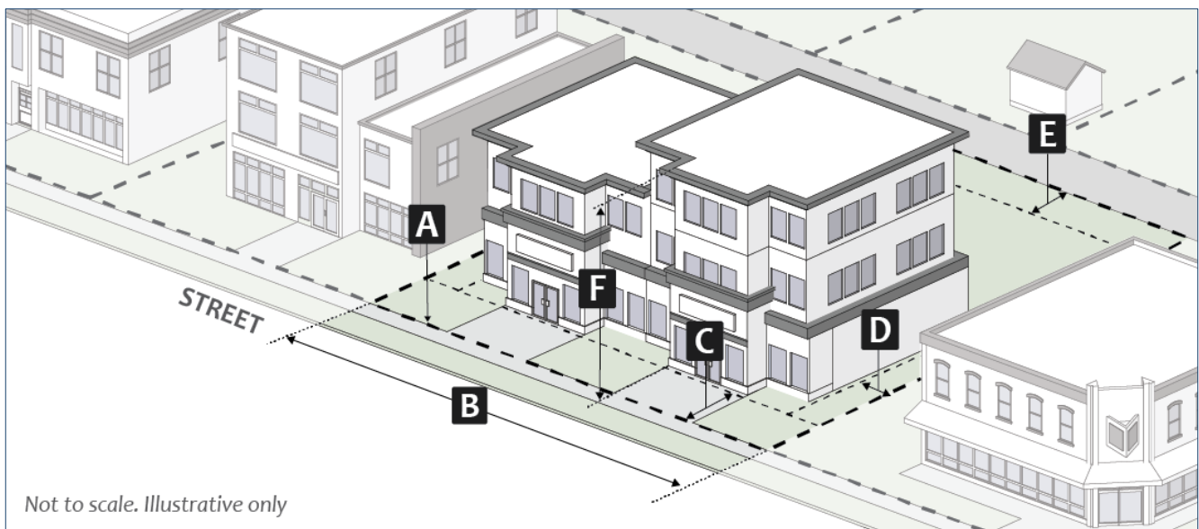
Figure 18: MN Dimensional Standards
